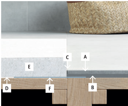
Floor installation
